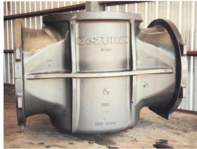
Gray Iron 60.50" Eccentric Flange Valve Body (A 126 Class B) - 21,000 pounds.
