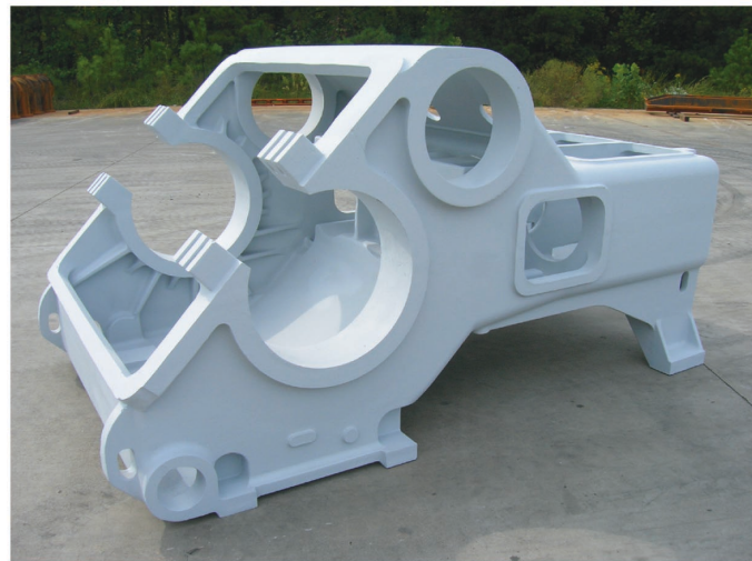
Ductile Iron (80/55/06) Slurry Pump Frame - 7540 pounds.
