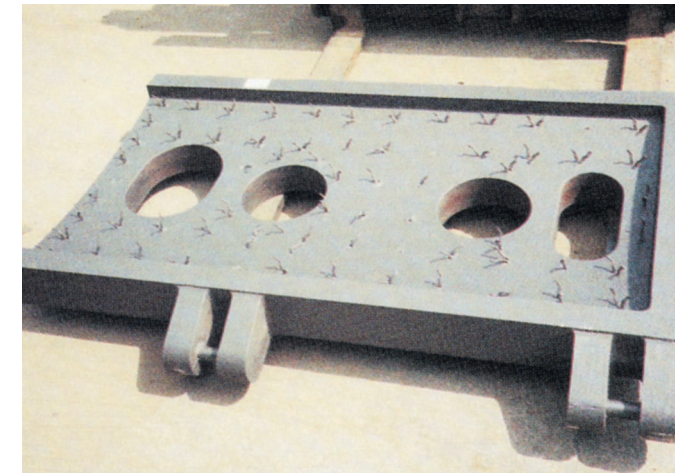
Ductile Iron Tundish Cover (60/40/18) with Stainless Steel Refractory Anchors Cast In - 10,100 pounds.
