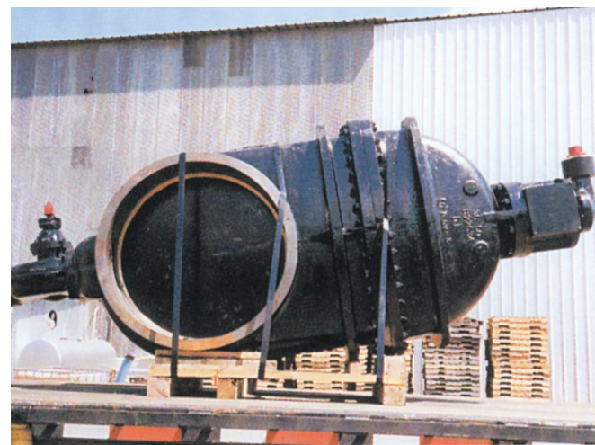
Ductile Iron 36" Double Disc Gate Valve (65/45/12), machined and assembled - 8830 pounds.
